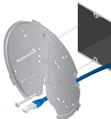
Junction or Outlet Box Mount Option
